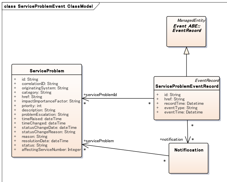
Figure 3 - Service Problem Event Record resource model
