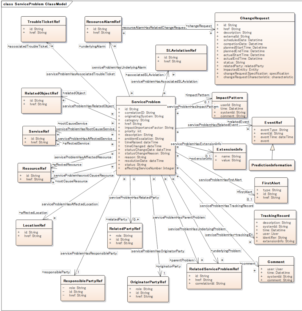
Figure 1 – Service Problem resource model
