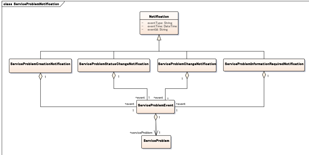
Figure 4 – Service Problem Notification Resource model
