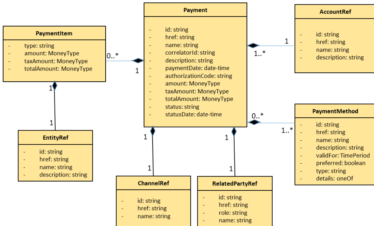
Figure 1 Payment resource model
