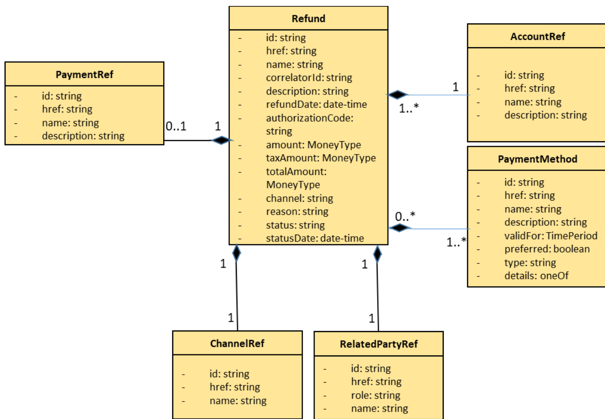
Figure 2 Refund resource model
